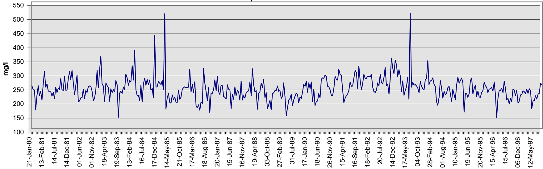
Dissolved Suspended Solids Mile 847.7
