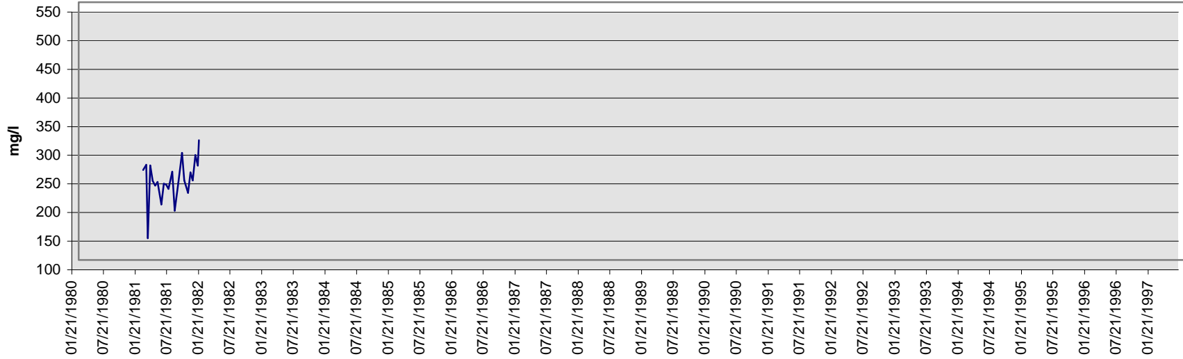
Dissolved Suspended Solids Mile 847.7
