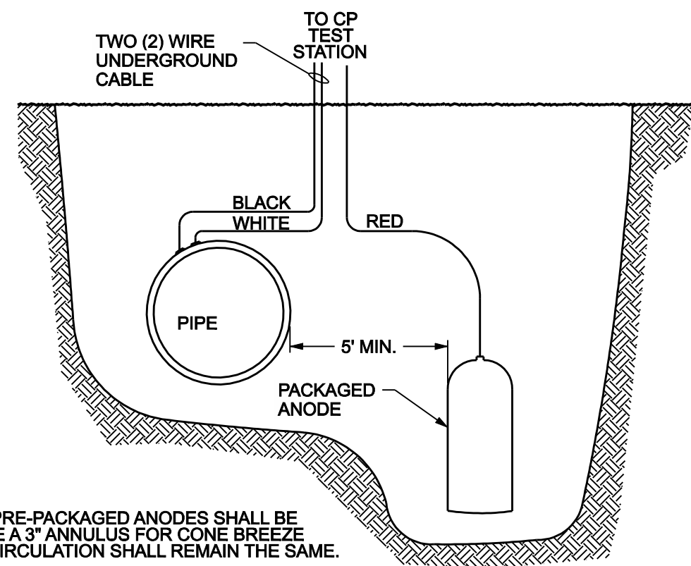
SINGLE ANODE INSTALLATION WITH TEST LINES
