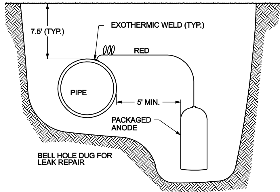
SINGLE ANODE INSTALLATION
