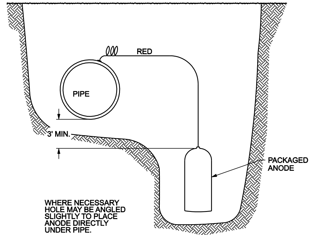
UNDER PIPE ANODE INSTALLATION
