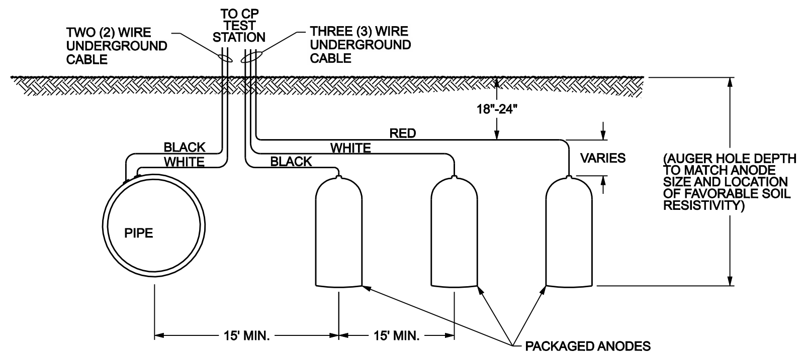
MULTIPLE ANODE INSTALLATION WITH TEST LINES
